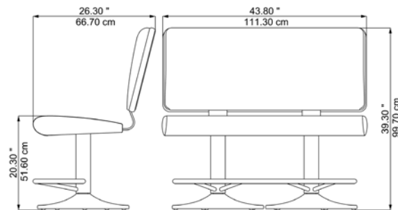
DOUBLE PEDESTAL BASE
