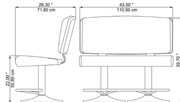
DOUBLE PEDESTAL BASE
